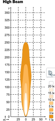
N4407 QD, N4408, 3500lm High Beam
